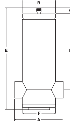
Air Separator
