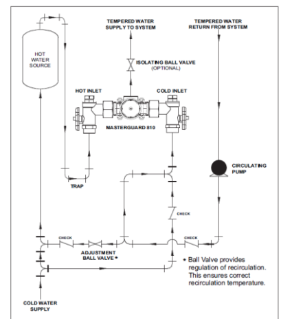
RECIRCULATION PIPING DIAGRAM
